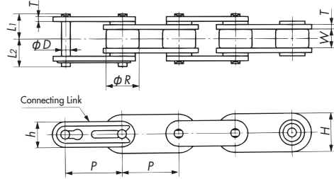
Stainless Steel Chain
