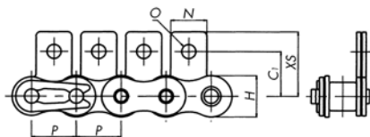
WK1, WK2 Attachments
