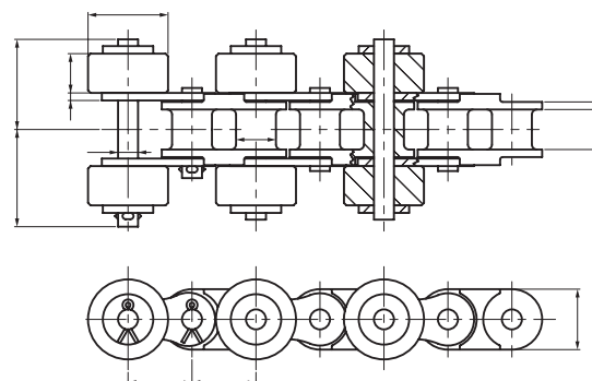
Crosswise Installation (Type II)
