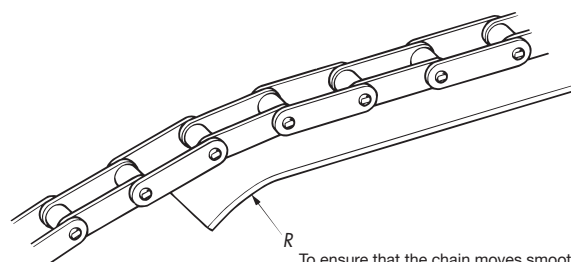
Figure 4: Rail Joints
