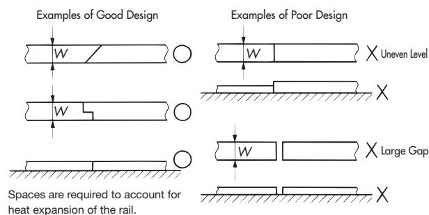
Figure 4: Rail Joints
