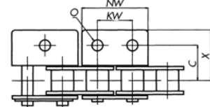
WA1, WA2 Attachments
