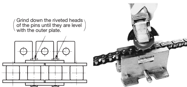
Figure 6: Attachment Chain
